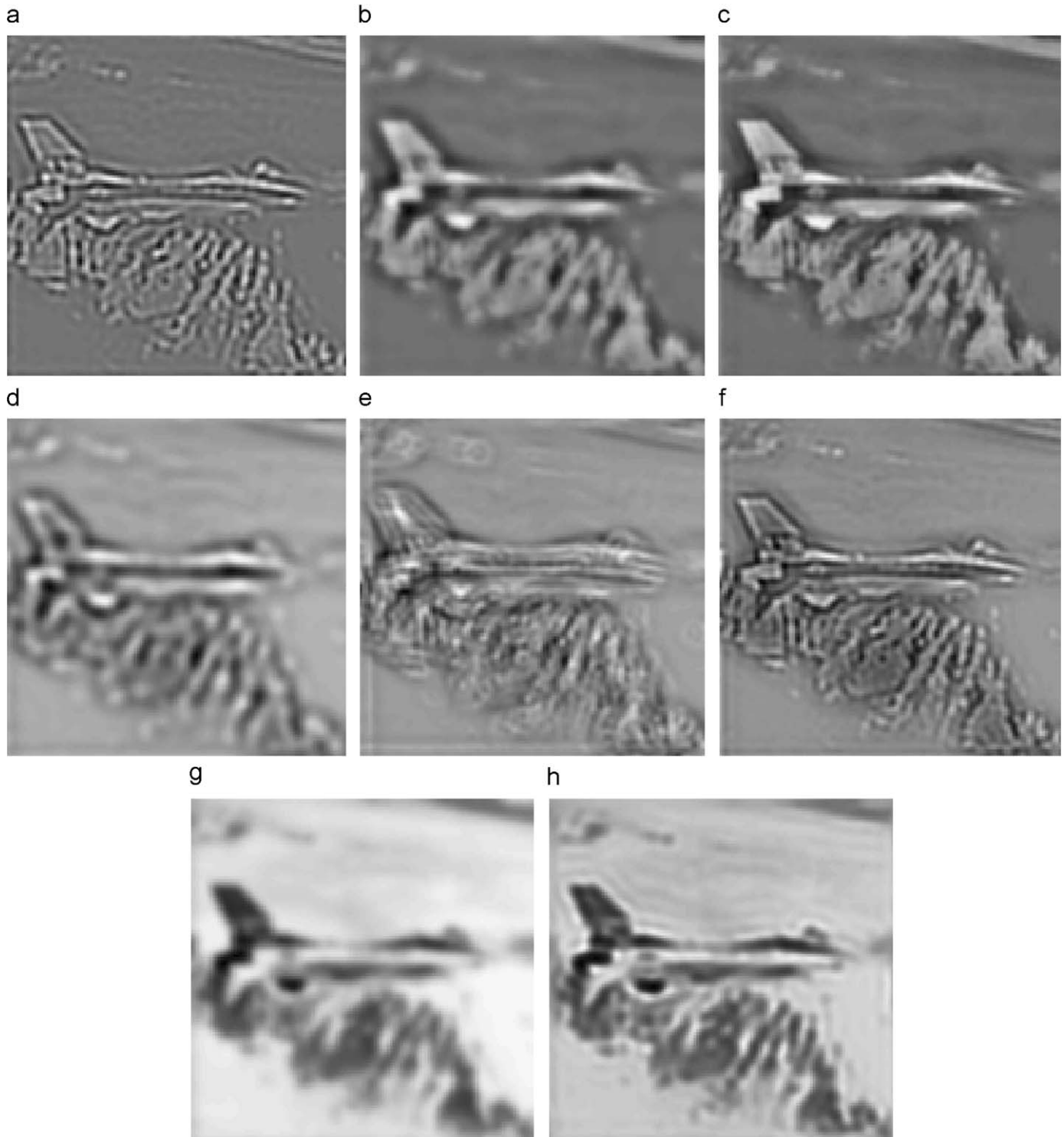
Fig. 3. Images restored from four simulated blurred frames using (a) ICA (JADE), (b) DCA (IN-JADE), (c) DCA (HP-JADE), (d) DCA (SDICA), (e) ISA, (f) NMF, (g) NTF, and (h) BRL algorithms.
