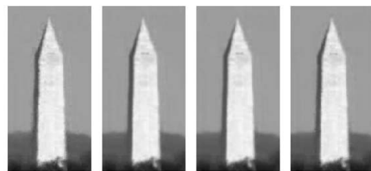
JADE HP-JADE IN-JADE SDICA Givens Rotation: (9341) (4931) (3912) (123) Laplacian Metric: (1.9220) (1.4408) (1.4328) (1.6084)
