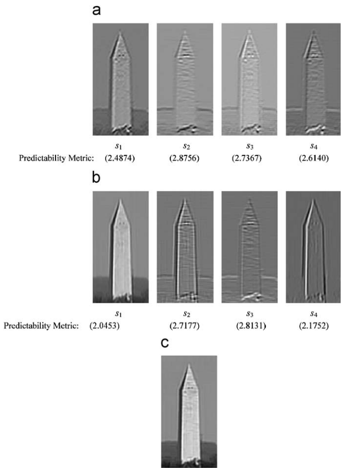
Fig. 15. Image enhancement for Fig. 13 using single-frame multi-channel filtering: (a) Gabor+Wavelet+ICA (4 sources), (b) Gabor+Innovation+ICA (4 sources) and (c) Gabor+Innovation+ICA (1 source).
