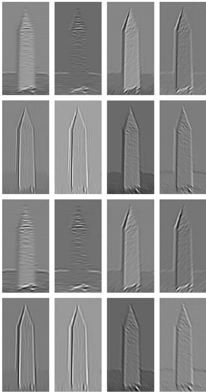
Fig. 14. Multi-channel version of the original image in Fig. 13 produced by the 2D Gabor filter bank with two spatial frequencies and four orientations.
